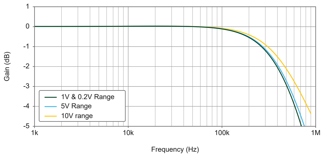
Figure 3 : USB-6421 Small Signal Bandwidth versus Frequency
