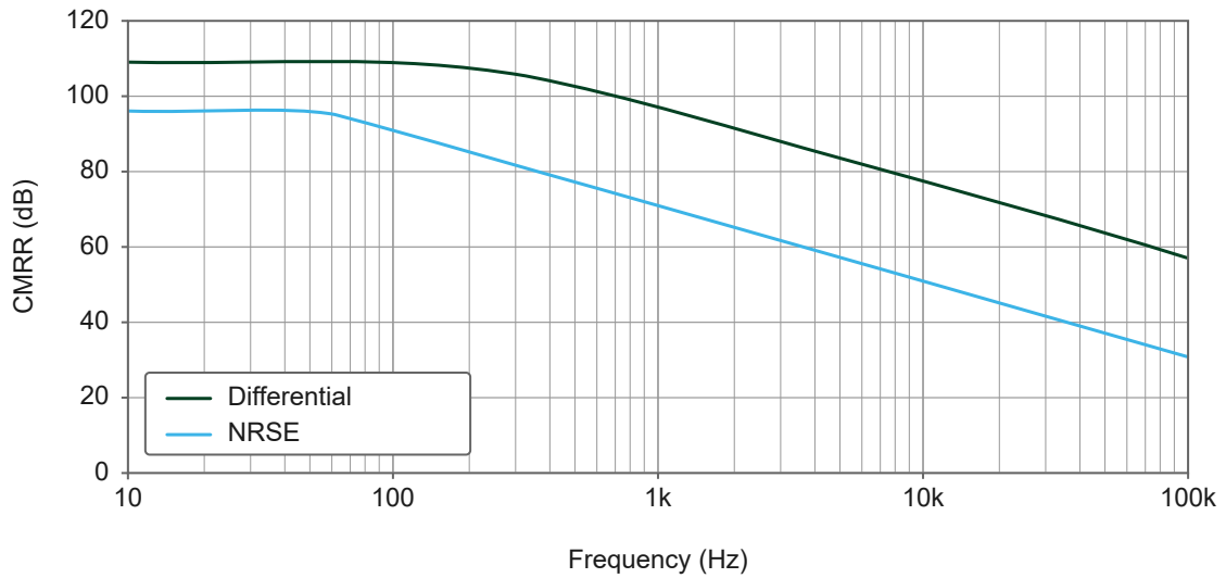
Figure 4 : USB-6421 CMRR versus Frequency
