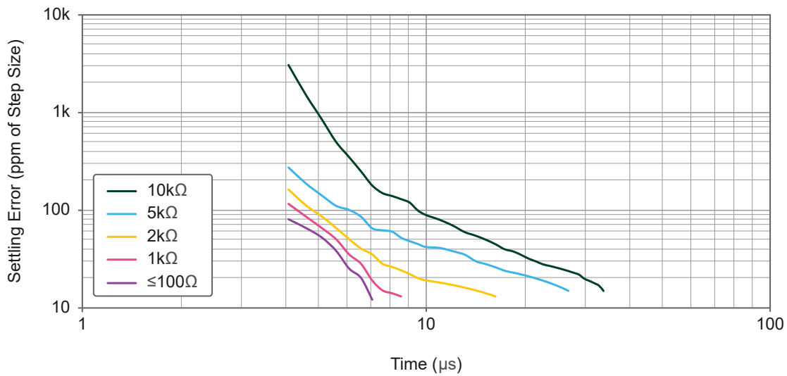
Figure 5 : USB-6421 Settling Error versus Time for Different Source Impedances
