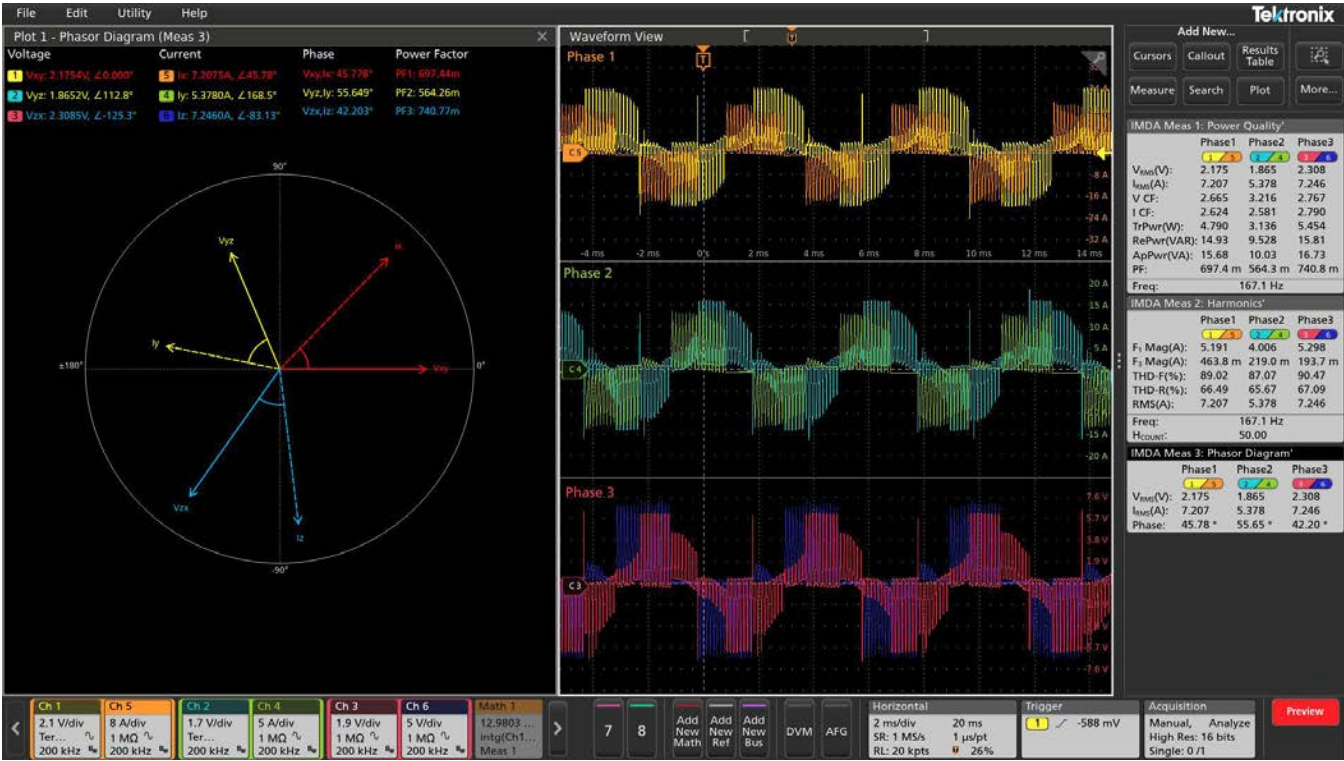
On the left is a Phasor Diagram displaying the phase and magnitude of current and voltage measurements for all three phases of power. In the results badge on the right, are the results from the automated measurements of power quality, power harmonics and the phasor diagram.
