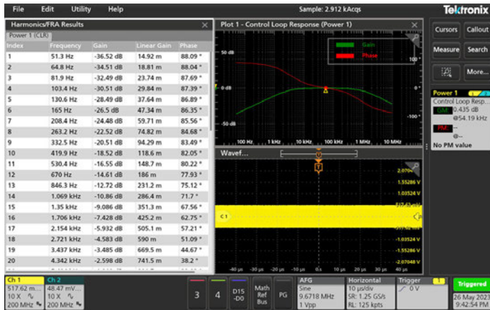
Frequency Response Analysis on the 2 Series MSO.
