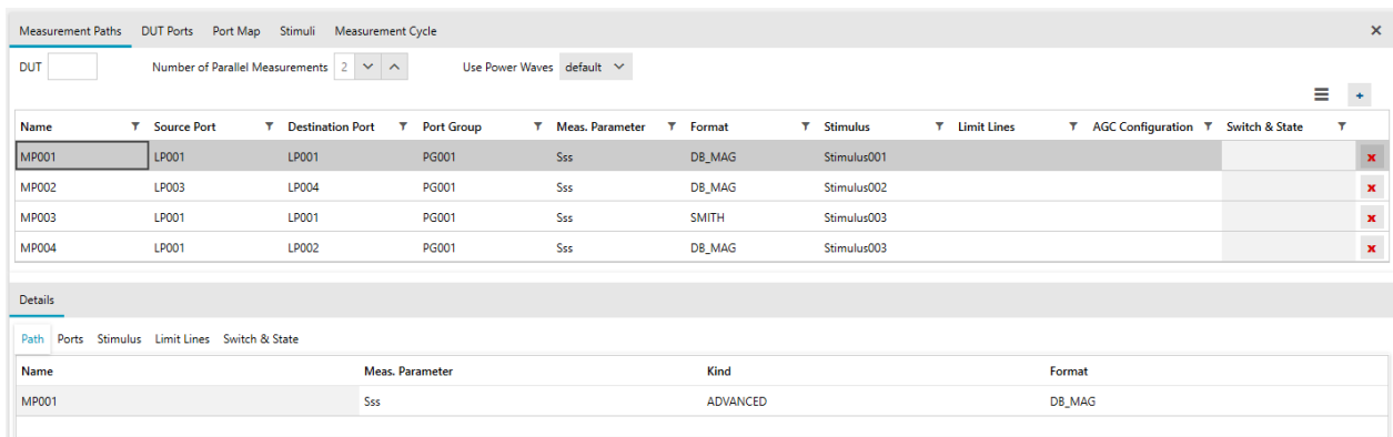
Figure 4-3: Populated workspace
