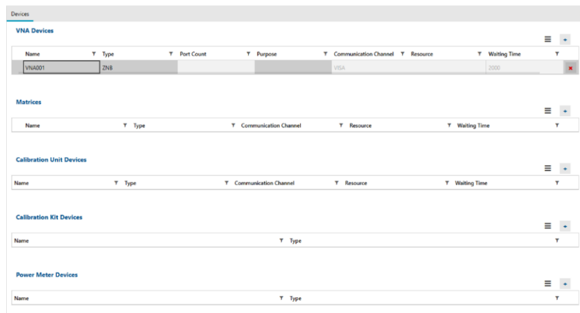
Figure 4-35: Devices workspace
