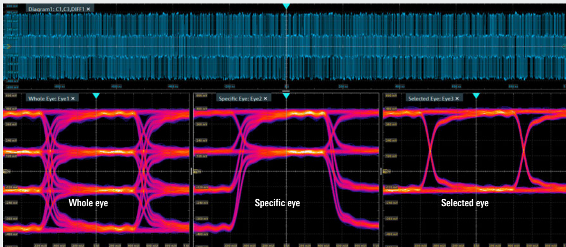
PAM-3 signal analysis: Eye diagram display with whole, selected and specific filter mode
