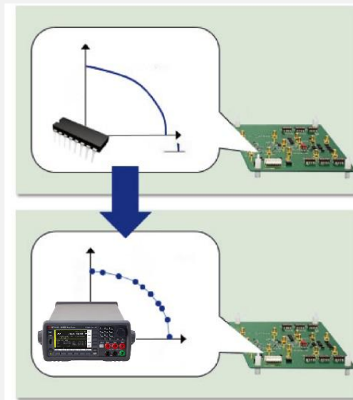
Figure 16. The B2961B/B2962B can emulate the DC voltage/current output characteristics of many devices and samples
