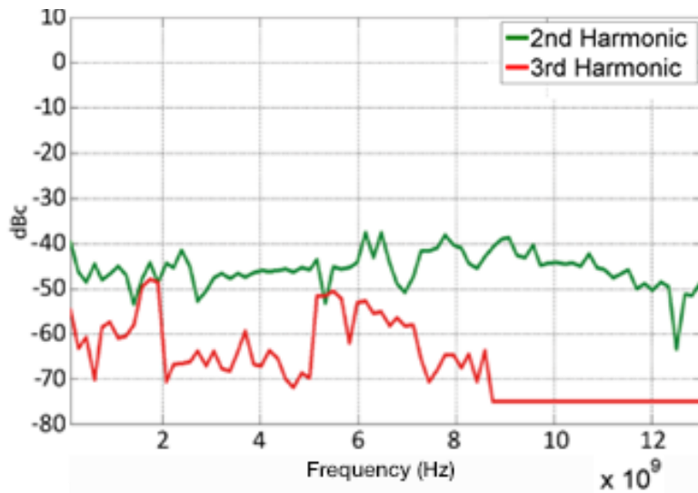
Figure 6. Typical harmonics
