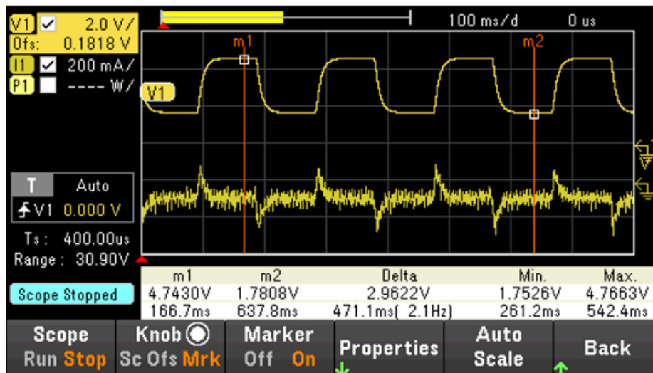
Figure 10. Scope View.
