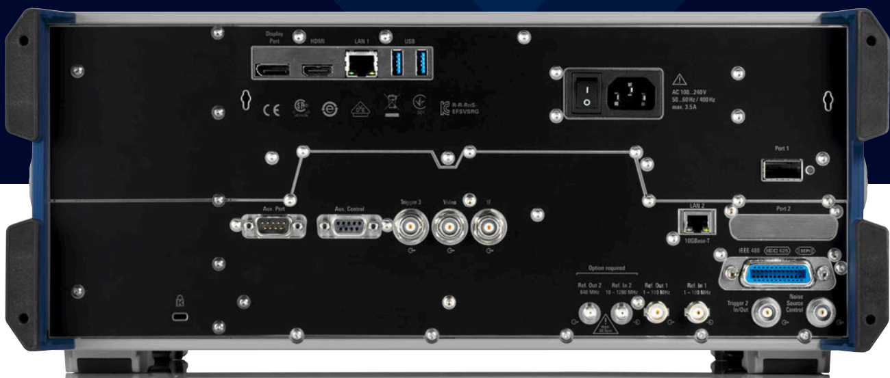
Rear view of the R&S®FSVA3000.
