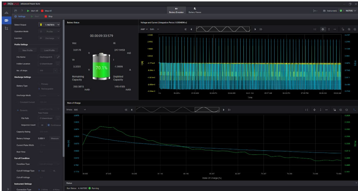
Figure 8. PW9253A creating a battery model with dynamic profile function
