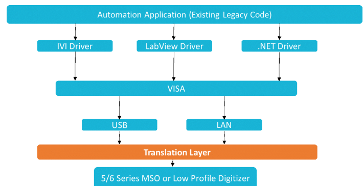
How the PI Translator works from Automation software to Tek instrument
