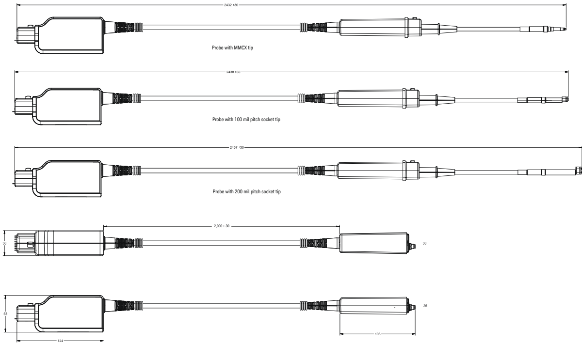
Figure 15 PP0004A/6A/8A Probe Dimensions
