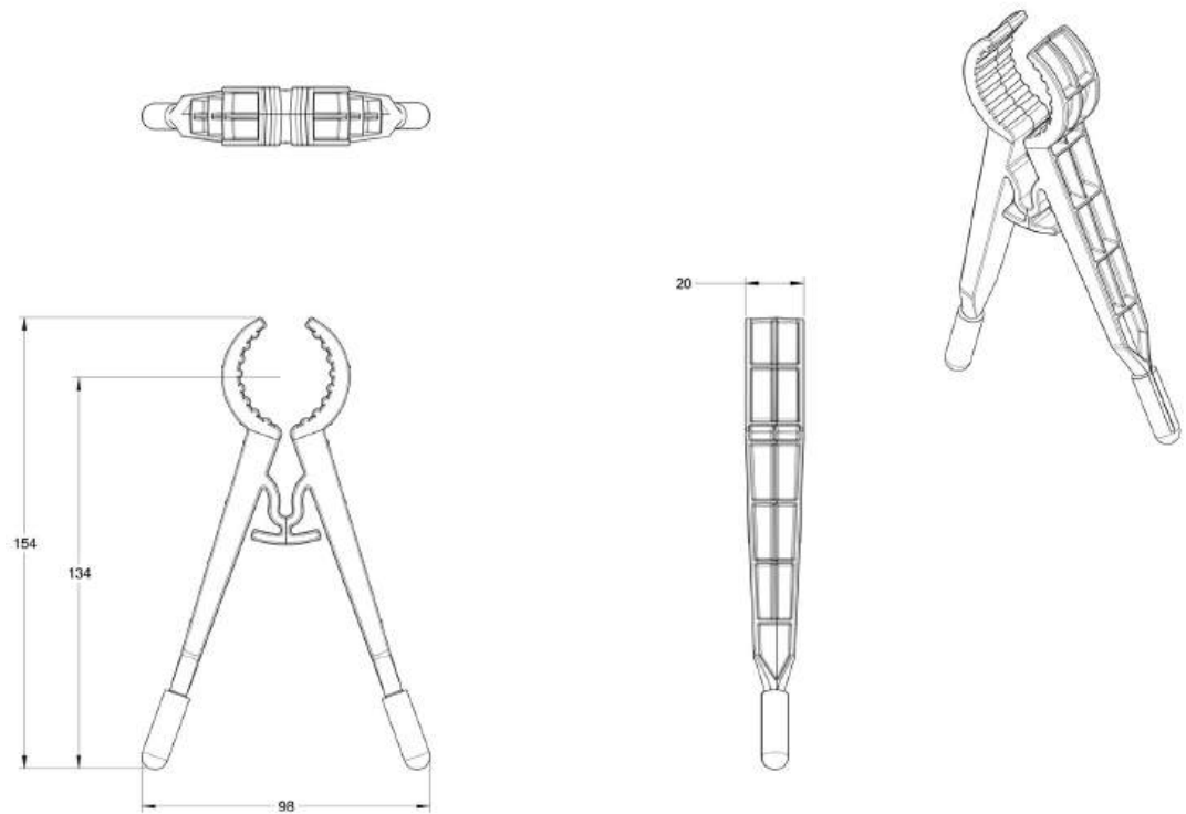
Figure 19 Bipod Dimensions
