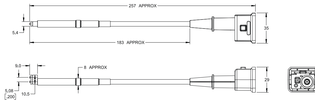
Figure 18 200 Mil Pitch Socket Probe Tip Dimensions
