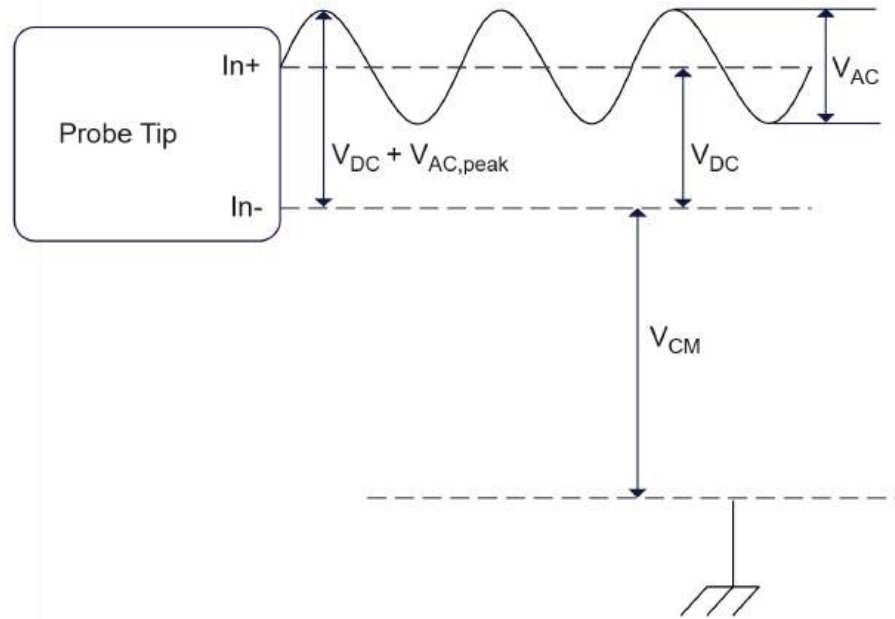
Figure 8 Input Voltage Terms
