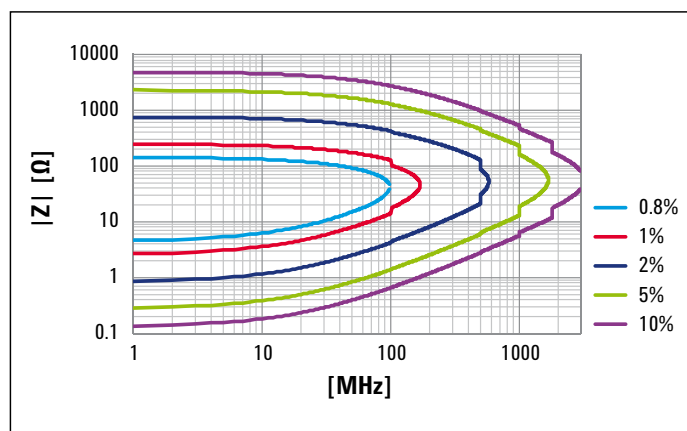
Figure 4. Measurement Time: Mode 3, Oscillator Level = 1 dBm, Averaging Factor \geq 8 , Temperature Deviation \leq 5^\circ\text{C}
