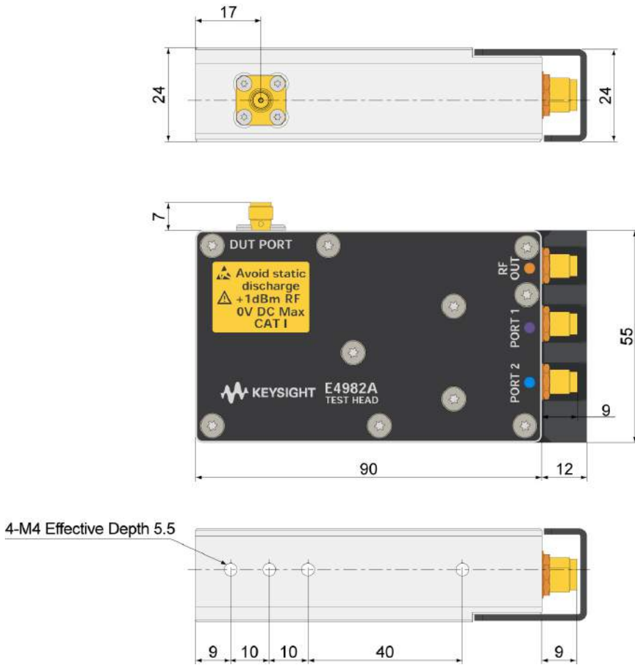
Figure 15. Test head.
