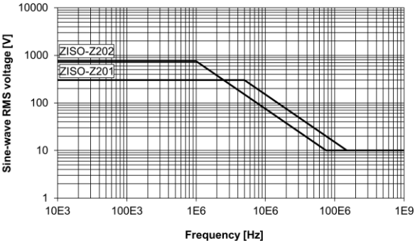
R&S®ZISO-Z201/-Z202 maximum rated sine-wave root mean square voltage between probe tip and probe reference terminal versus frequency (CAT III)
