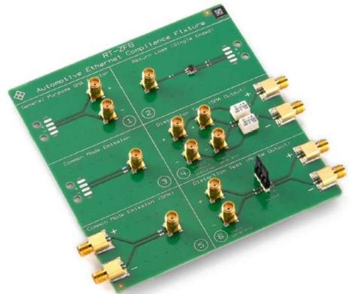
R&S®RT-ZF8 automotive Ethernet compliance test fixture
