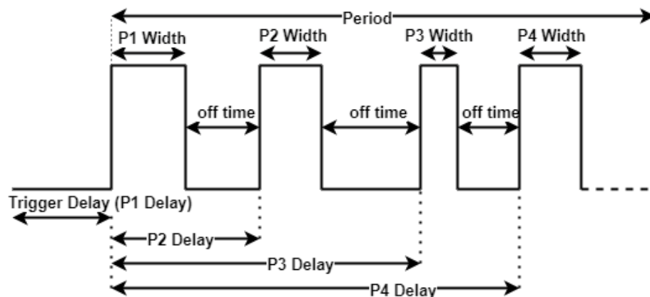
Figure 8. N-Pulse modulation
