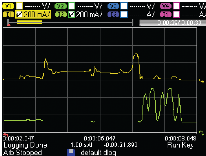
Figure 5. In Data Logger View, you can log data on multiple traces. Here, the current flowing out of output 1 and output 2 is captured over 30 seconds.
