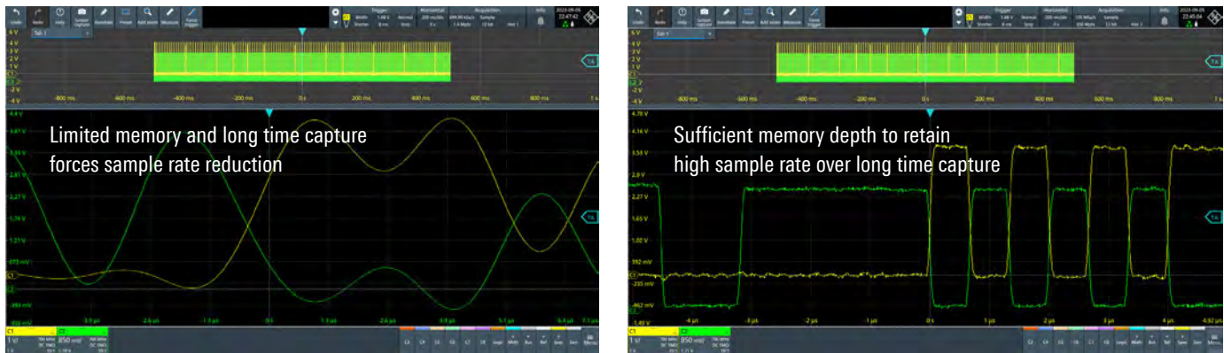
Fig. 4: More memory means the instrument can capture more time without reducing the sample rate
