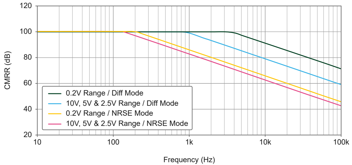
Figure 4: USB-6453 CMRR versus Frequency
