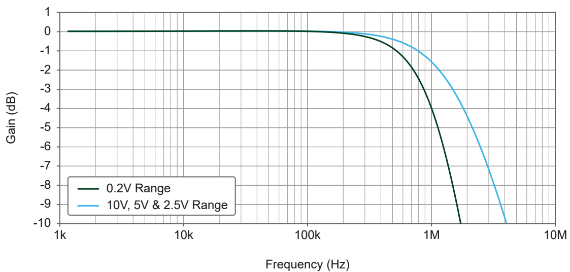
Figure 3 : USB-6453 Small Signal Bandwidth versus Frequency
