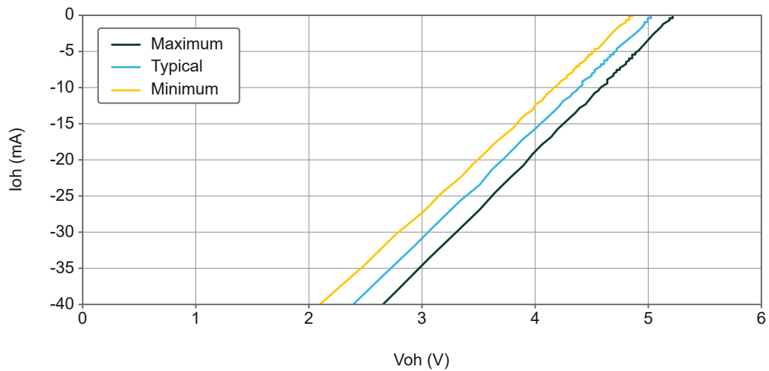
Figure 7 : I_{OH} versus V_{OH} , 5.0 V Logic Family
