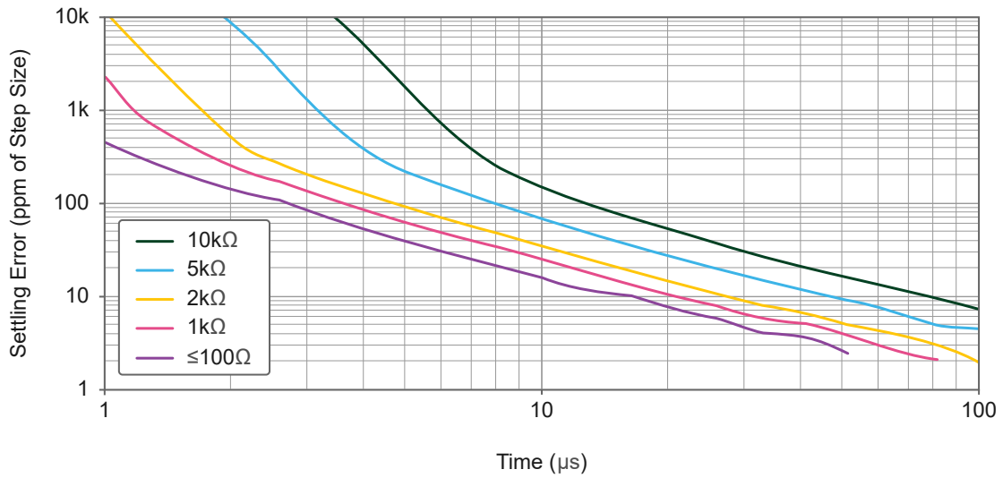
Figure 5 : USB-6451 Settling Error versus Time for Different Source Impedances at 10 V, 5 V, and 2.5 V Input Ranges
