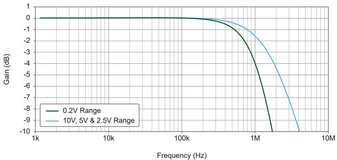
Figure 3 : USB-6451 Small Signal Bandwidth versus Frequency
